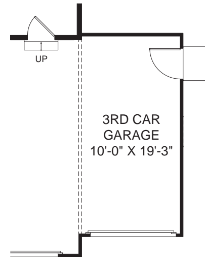
Optional 3rd Car Garage (Shown with Optional Service Door)
