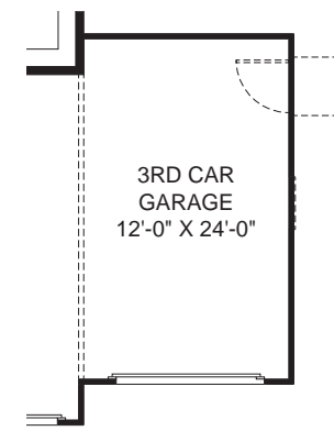
Optional 12' x 24' 3rd Car Garage Stall
