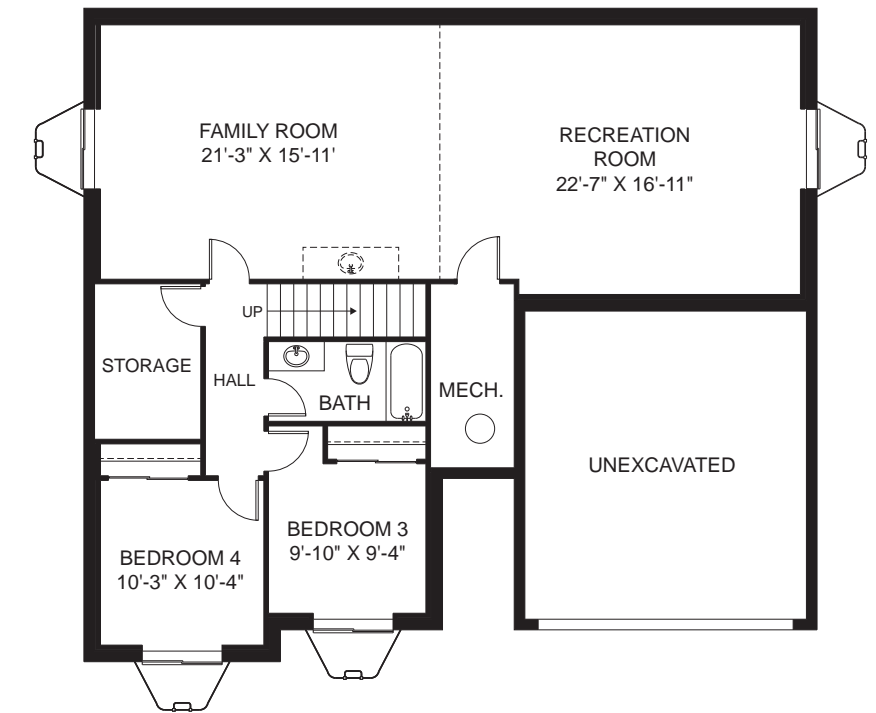
Optional Finished Basement (Shown with Optional Additional Basement Window)
