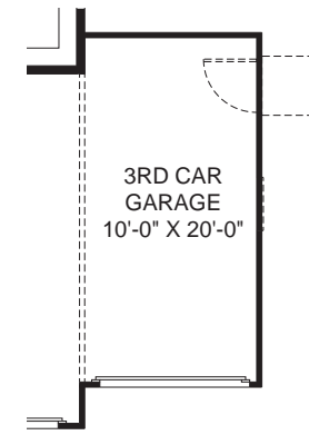
Optional 10' x 20' 3rd Car Garage Stall
